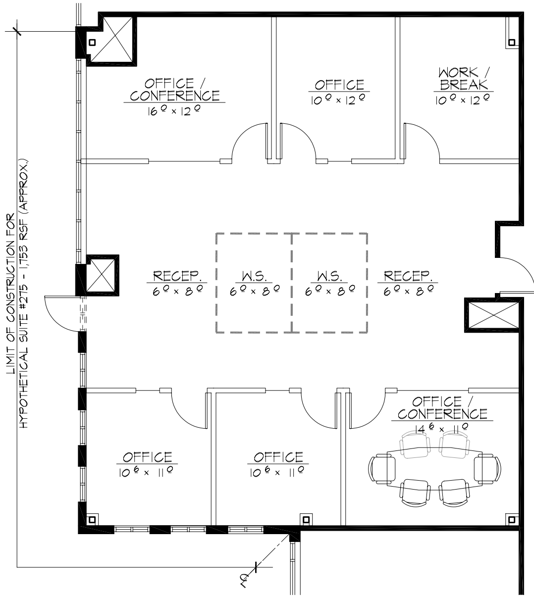
PRELIMINARY SPACE PLAN #1 SCALE: 1/8" = 1'-0"
